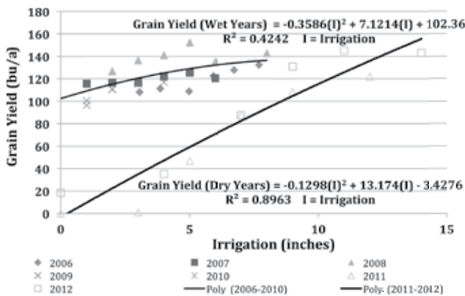
Figure 2. Yield response of grain sorghum at various levels of irrigation at Garden City, KS shown by years. Years 2006 – 2010 are near average or above precipitation (wet) years. 2011 – 2012 are drought (dry) years.
