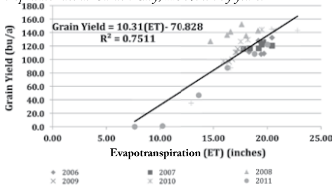
Figure 1. Yield response of grain sorghum at various levels of crop water use at Garden City, KS shown by years.
